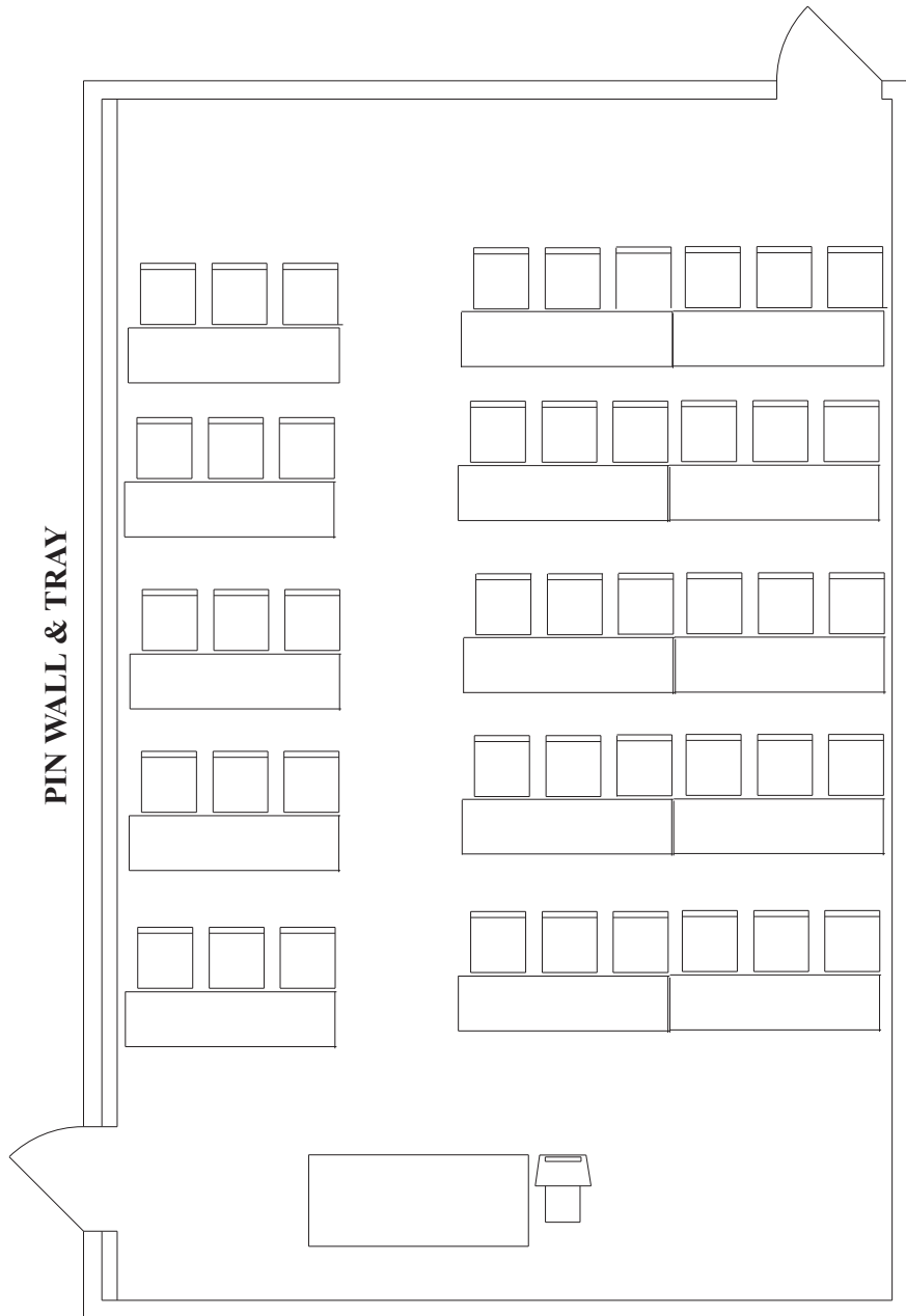
WALT DISNEY WORLD DOLPHIN EUROPE 8 AREA 706 SQ. FT. CEILING 11 FT. 10 IN. LOWEST PT. 11 FT. 1 IN. Schoolroom 0 2 5 3/16" = 1' 45 Chairs
